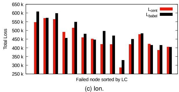
Figure 6. Comparison of the loss induced by the failure of the 15 more central nodes in ninux (a) Graz (b) and Ion (c) when standard Babel is used ( L_{babel} ) or the modified version is used ( L_{cent} )
