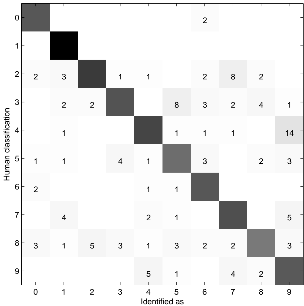
Confusion matrix for digits using L2-norm, nearest-neighbor
