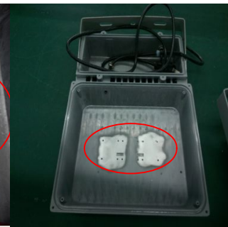
LED chip installed on polished board, good for heat emission from LED lighting source
