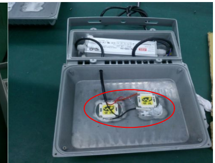
LED chip installed on polished board, good for heat emission from LED lighting source
